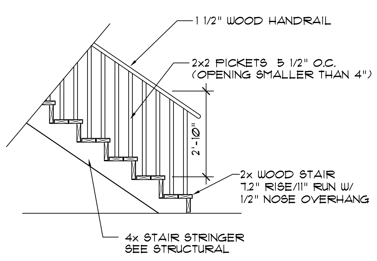
TYPICAL STAIR DETAIL SCALE: 1/2" = 1'-0"
